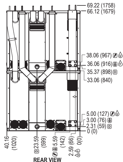
REAR VIEW
